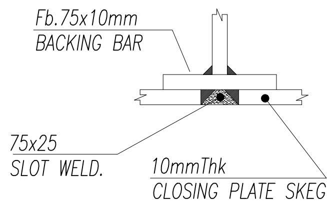
SECTION 'A-A' 1:10
