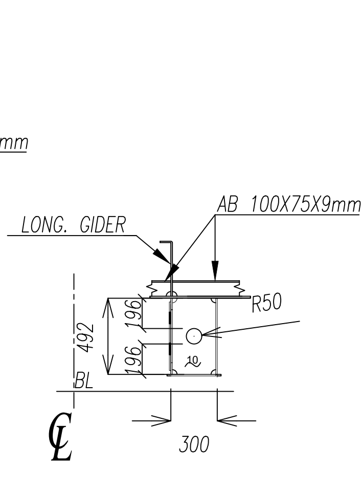
FRAME 2
