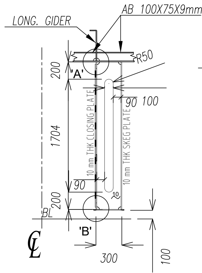
FRAME 0 +682
