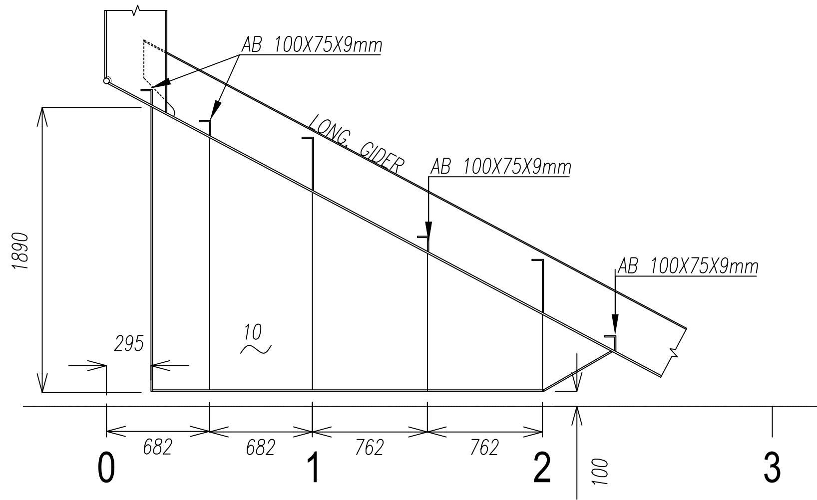
ELEVATION (OUT-SIDE)
