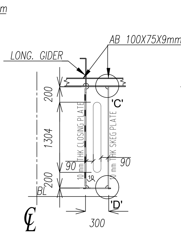
FRAME 1
